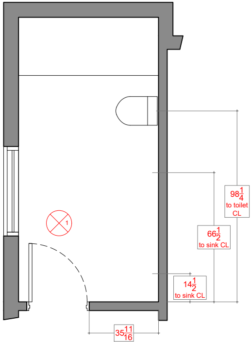
Plan
